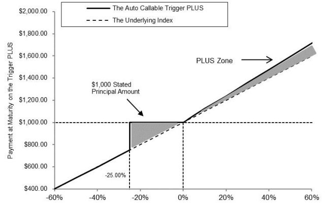
Auto-Callable Trigger PLUS Payoff Diagram*
