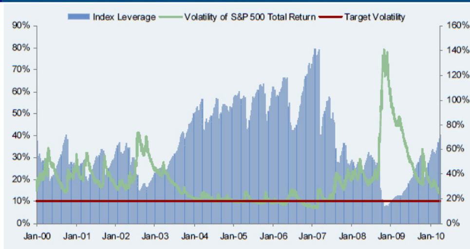
Hypothetical Index leverage and volatility (Jan 3, 2000 – Mar 31, 2010)
