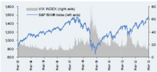
Historical performance comparison of the S&P 500® Index and the VIX Index: March 2003 – March 2013
