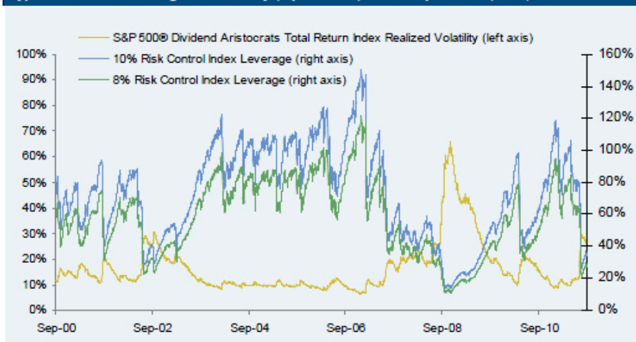
Hypothetical Index leverage and volatility (September 28, 2001 – September 30, 2011)
