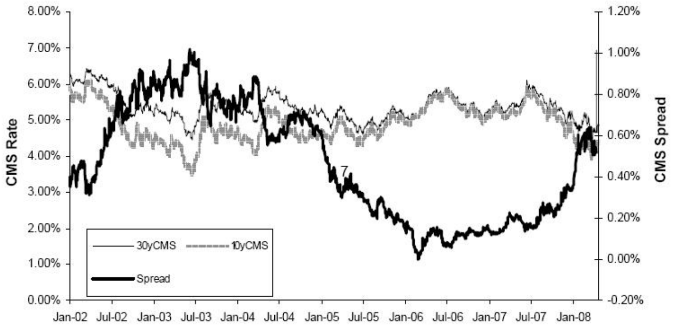
30-Year CMS Rate, 10-Year CMS Rate and CMS Spread
